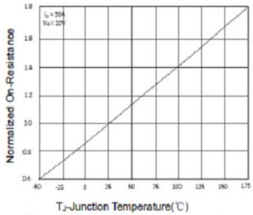
Figure 4 Rds(on)-Junction Temperature
