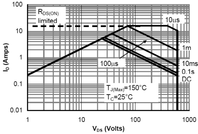
Figure 9: Maximum Forward Biased Safe Operating
