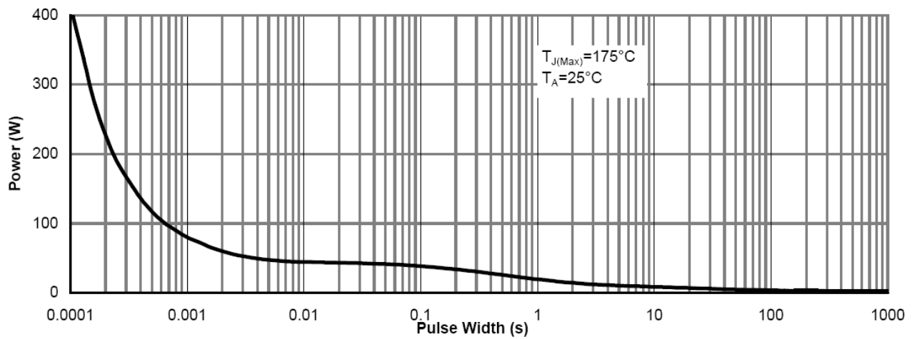
Figure 14: Single Pulse Power Rating Junction-to-Case (Note G)
