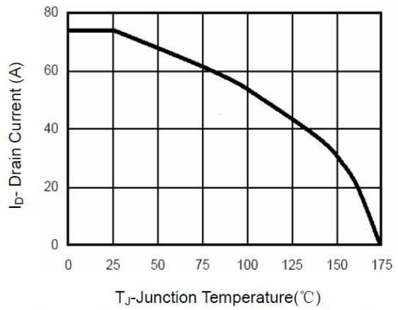
Figure 9 ID Current Derating vs Junction Temperature
